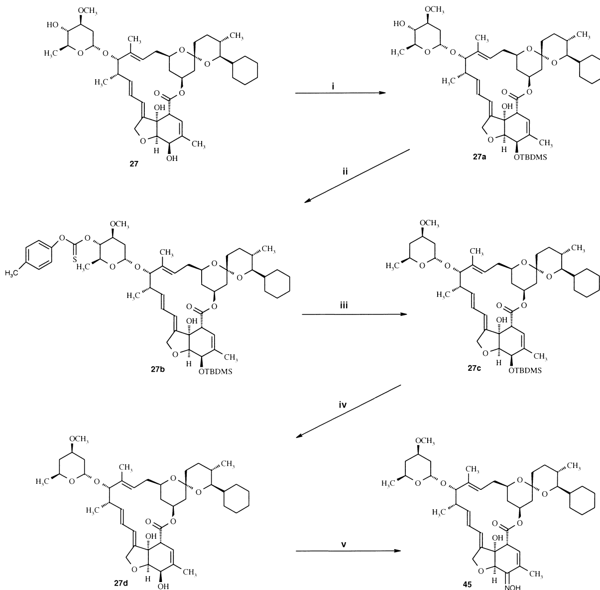
Scheme 2. Synthesis of oxime 45 . Reagents and conditions: i. 1.43 equiv of tert -butyldimethylsilyl chloride, 2.2 equiv of imidazole, dimethylformamide, 25 °C, 3.5 h, 60%; ii. 2 equiv of para -tolyl chlorothionoformate, pyridine, dichloromethane, 25 °C, 3 h; iii. 89.2 equiv of tributyltin hydride, 0.01 equiv of 2,2'-azobis(isobutyronitrile), toluene, 110 °C, 1 h; iv. 1.31 equiv of para -toluenesulphonic acid, methanol, 25 °C, 35% over 3 steps; v. (a). manganese dioxide, diethyl ether, 25 °C, 22 h; (b). 11.7 equiv of hydroxylamine hydrochloride, methanol, dioxan, water, 25–40 °C, 4 h, 76% over 2 steps.
